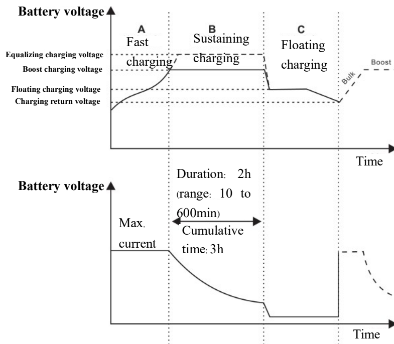
Fig. 1-5 Battery charging stages diagram
