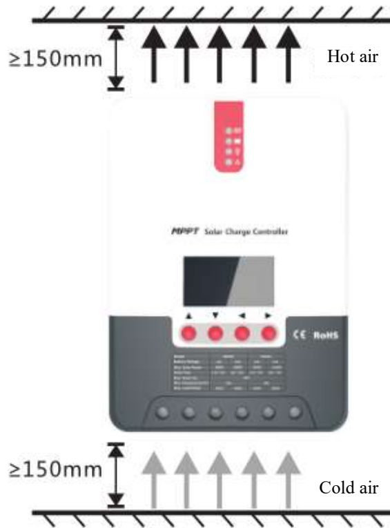
Fig. 2.1 Installation and heat dissipation
